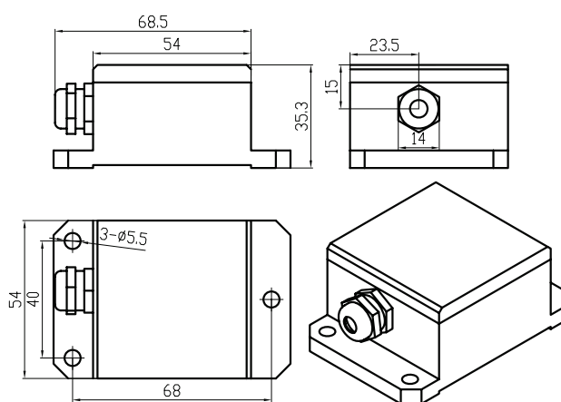
Picture 4 SST100 with metal pigtail
